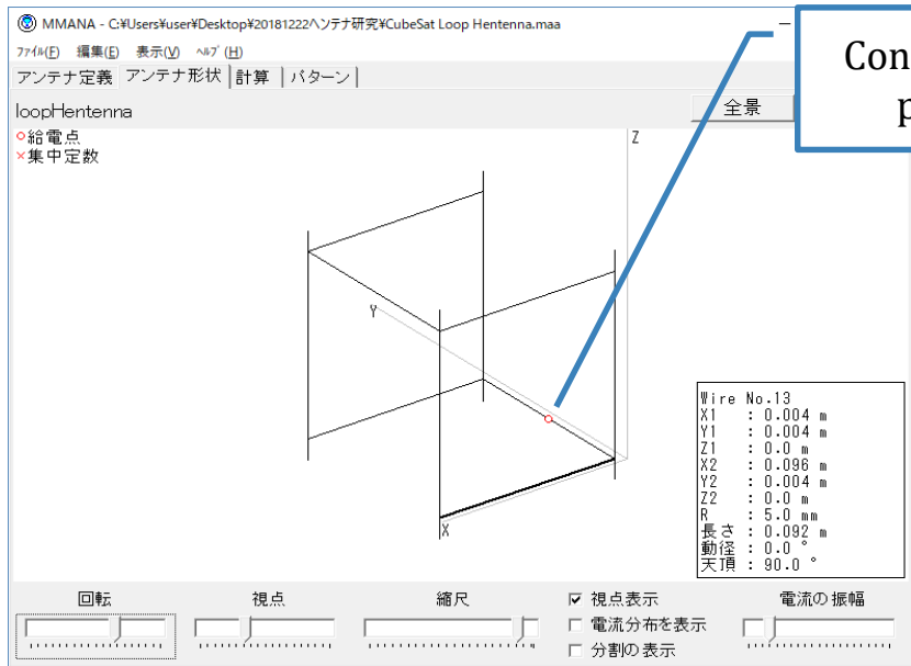
Structure of Loop Hentenna
