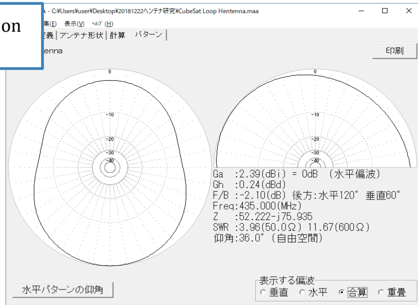
Antenna Pattern of Loop Hentenna
