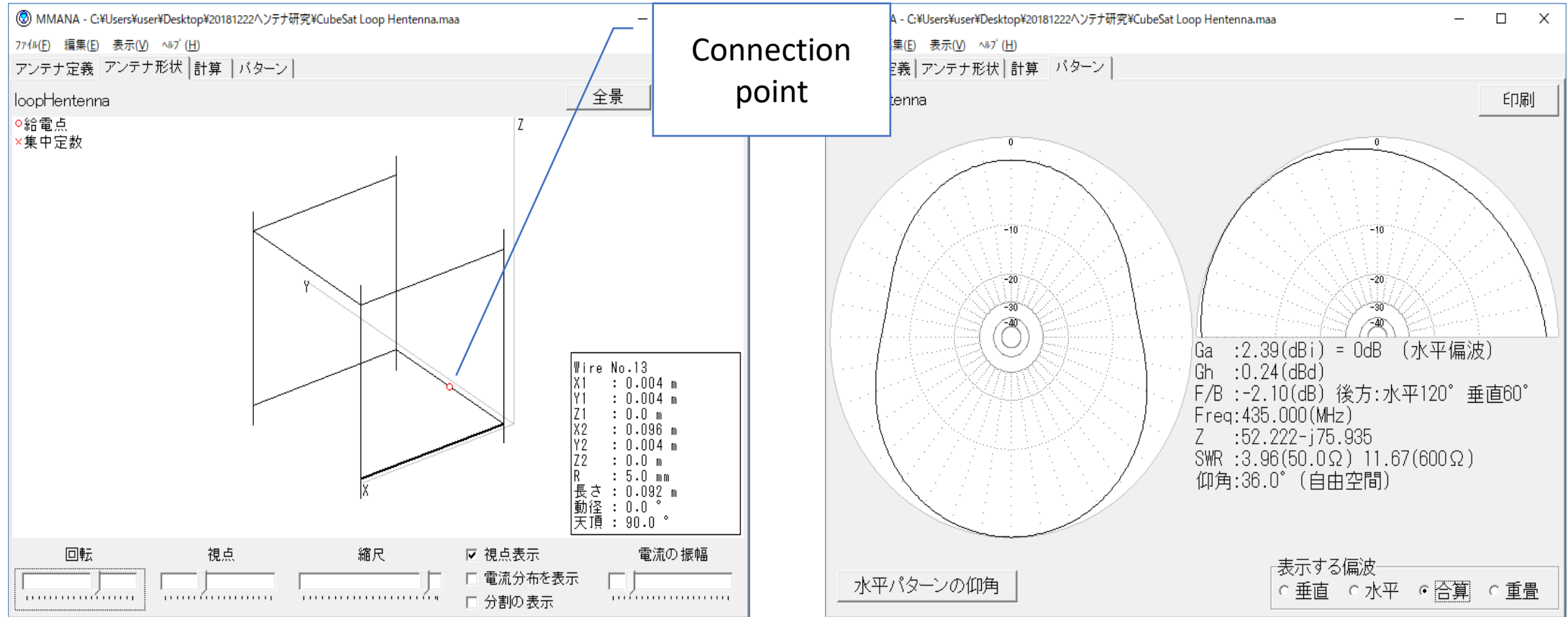
Structure of Loop Hentenna
